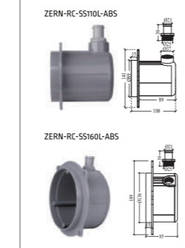
Plastic niche for concrete pool
