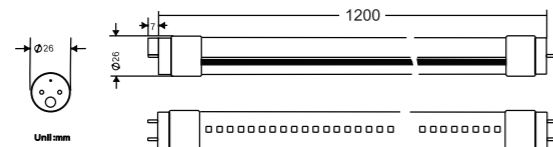
Dimension ( mm )
