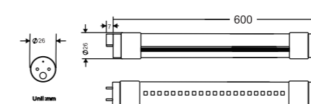
Dimension ( mm )
