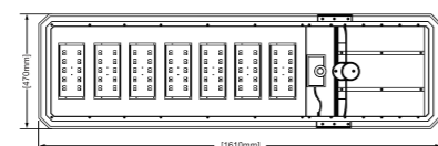
Dimension ( mm )
