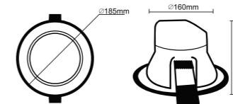
Dimension ( mm )
