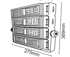
Dimension ( mm )
