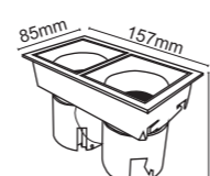
Dimension (mm)
