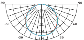
Light Distribution Curve
