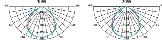
Light Distribution Curve
