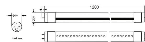
Dimension ( mm )
