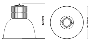
Dimension (mm)
