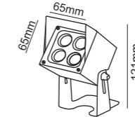
Dimension [ mm ]
