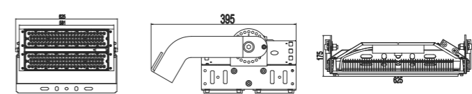
Dimension [ mm ]
