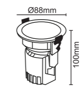
Dimension ( mm )
