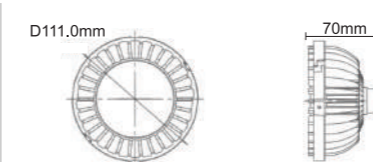
Dimension ( mm )
