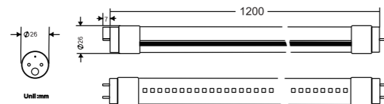
Dimension ( mm )
