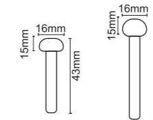
Dimension ( mm )
