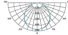
Light Distribution Curve
