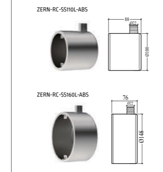
Stainless steel niche for concrete pool
