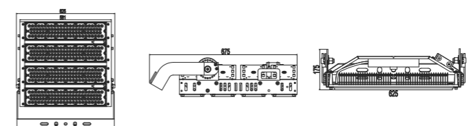
Dimension [ mm ]
