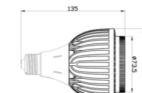
Dimension ( mm )
