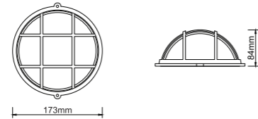
Dimension ( mm )
