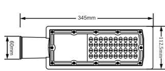
Dimension ( mm )
