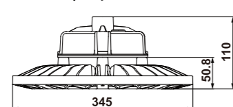
Dimension ( mm )
