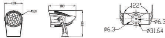
Dimension [ mm ]
