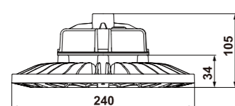
Dimension ( mm )
