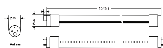
Dimension ( mm )
