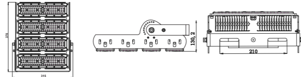
Dimension [ mm ]
