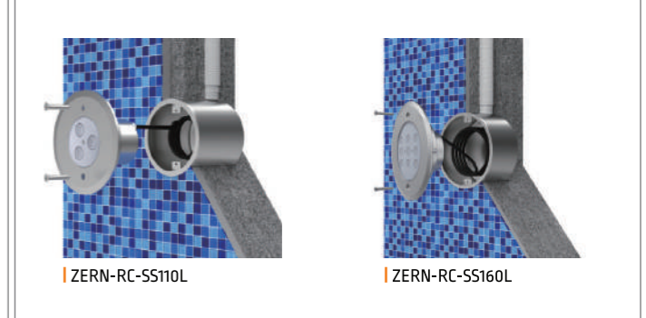
Installation Diagram
