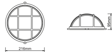
Dimension ( mm )
