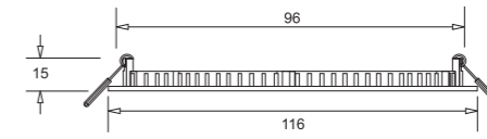
Dimension ( mm )
