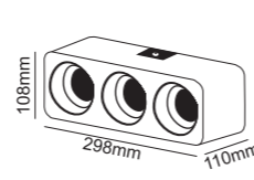
Dimension ( mm )
