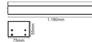
Dimension ( mm )
