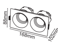
Dimension ( mm )
