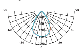
Light Distribution Curve
