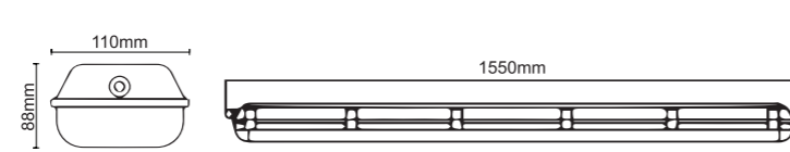
Dimension ( mm )
