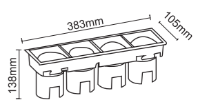
Dimension (mm)
