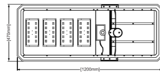
Dimension ( mm )
