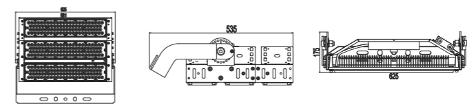
Dimension [ mm ]
