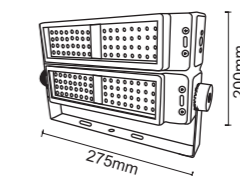
Dimension ( mm )
