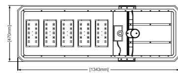
Dimension ( mm )
