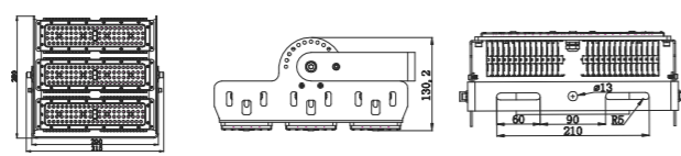
Dimension [ mm ]
