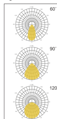
Light Distribution Curve
