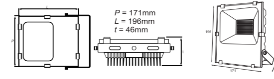
Dimension (mm)
