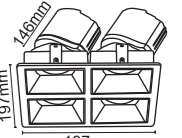
Dimension ( mm )
