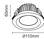
Dimension ( mm )
