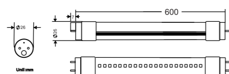
Dimension ( mm )
