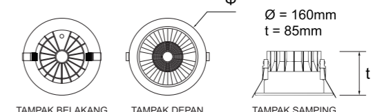
Dimension ( mm )
