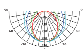
Light Distribution Curve
